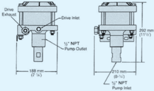
AFD or ASFD, -B60, -B100 pumps; double acting, high output
