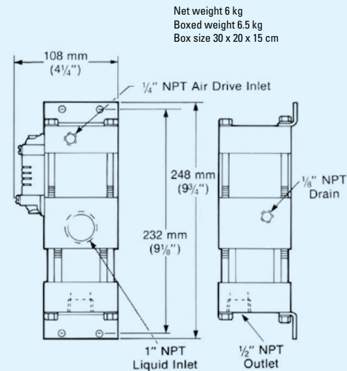
M-5 approx. weight 9 lbs (4 kg)
