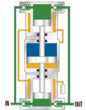
Model AGD Single Stage, Double Acting, Cooling Jackets
