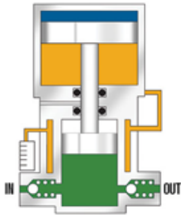
Model AG Single Stage, Single Acting
