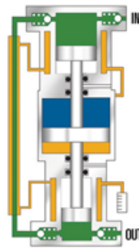
Model AGT Two Stage, Cooling Jackets
